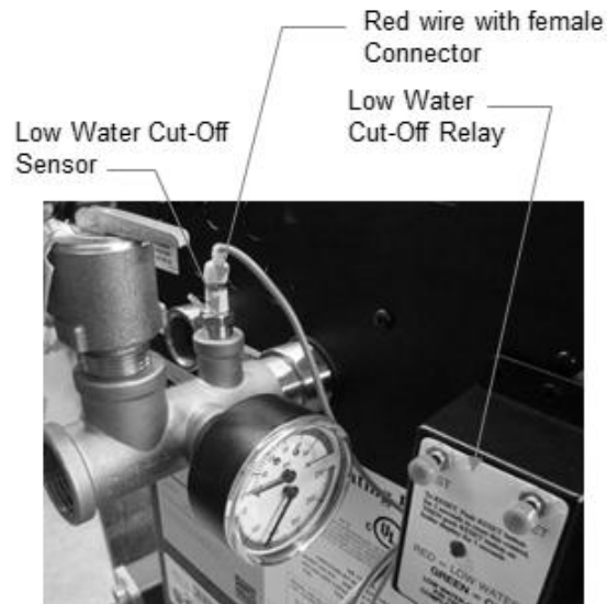
Figure 9– Low Water Cut-Off Detail
